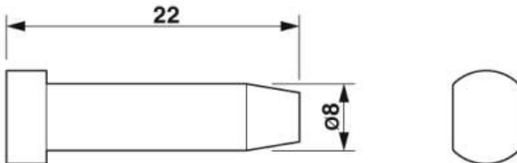
Dimensional drawing
