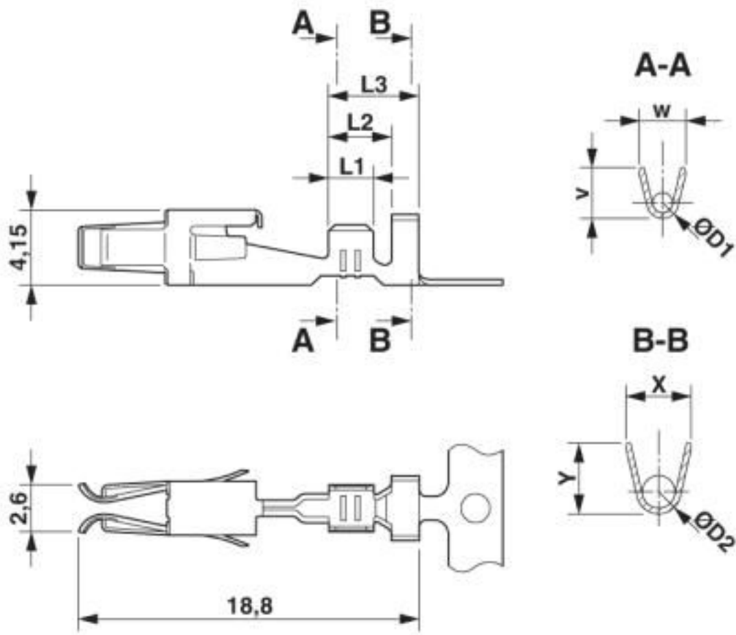
Dimensional drawing
