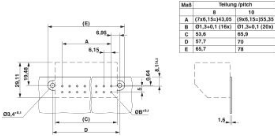
Dimensional drawing
