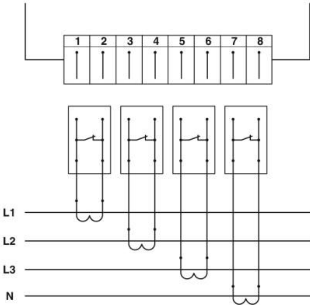
Circuit diagram
