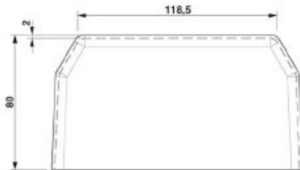
Dimensional drawing
