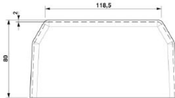
Dimensional drawing
