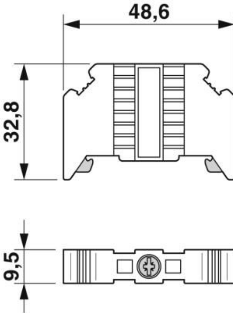
Dimensional drawing
