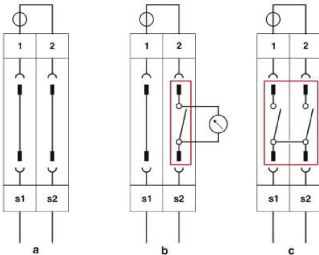
Circuit diagram
