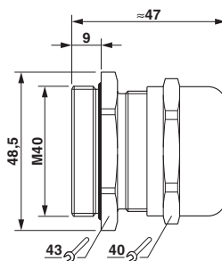
Dimensional drawing
