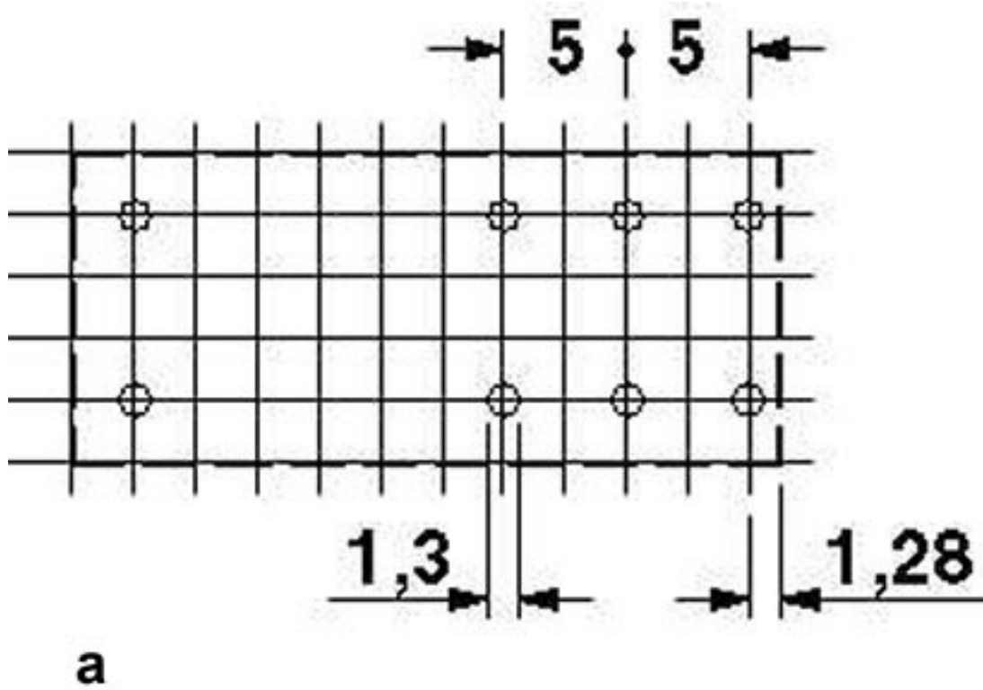
Drilling diagram
