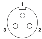
Socket, 3-pos.
