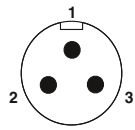
Plug, 3-pos.
