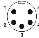
Plug, 5-pos.
