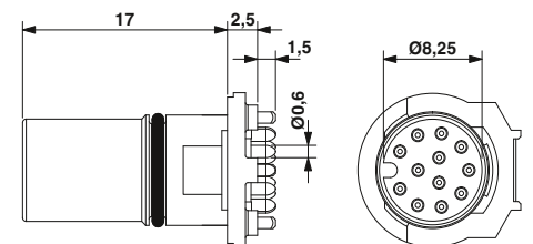
M12 socket contact carrier, straight, 12, 17-pos.
