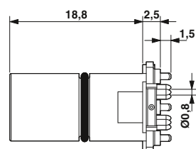
M12 plug contact carrier, straight, 8-pos.
