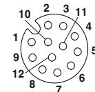
Socket, 12-pos.
