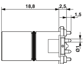
M12 plug contact carrier, straight, 4, 5-pos.
