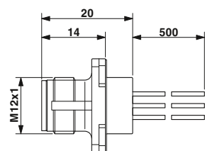
M12 flush-type plug, square flange
