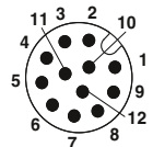
Plug, 12-pos.
