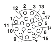
Socket, 17-pos.
