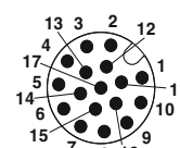
Plug, 17-pos.
