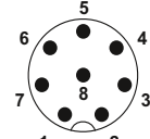
Plug, 8-pos.
