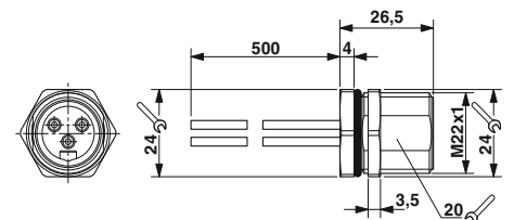
7/8" flush-type plug
