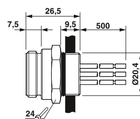
7/8" flush-type plug
