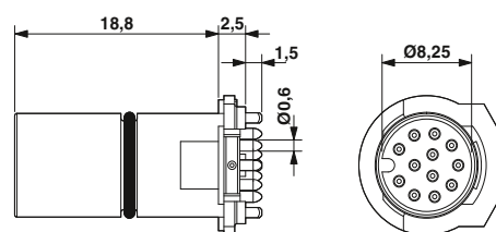
M12 plug contact carrier, straight, 12, 17-pos.
