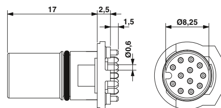
M12 socket contact carrier, straight, 12, 17-pos.
