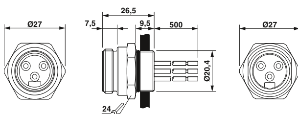
7/8" flush-type plug
