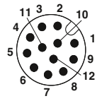
Plug, 12-pos.
