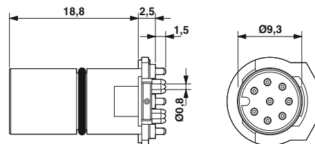
M12 plug contact carrier, straight, 8-pos.
