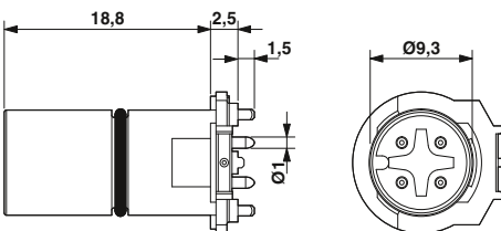
M12 plug contact carrier, straight, 4, 5-pos.
