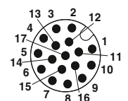
Plug, 17-pos.
