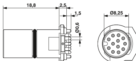
M12 plug contact carrier, straight, 12, 17-pos.
