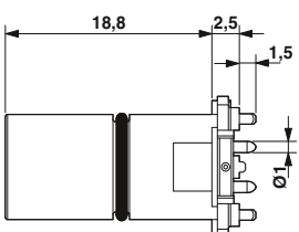
M12 plug contact carrier, straight, 4, 5-pos.
