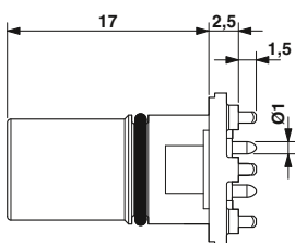
M12 socket contact carrier, straight, 4, 5-pos.
