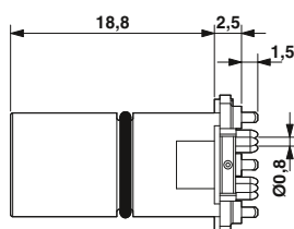
M12 plug contact carrier, straight, 8-pos.
