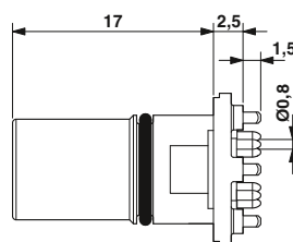
M12 socket contact carrier, straight, 8-pos.
