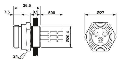
7/8" flush-type plug
