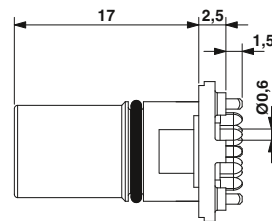
M12 socket contact carrier, straight, 12, 17-pos.
