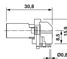
M12 pin contact carrier, angled, 17-pos.
