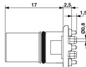
M12 socket contact carrier, straight, 8-pos.
