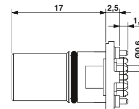
M12 socket contact carrier, straight, 12, 17-pos.
