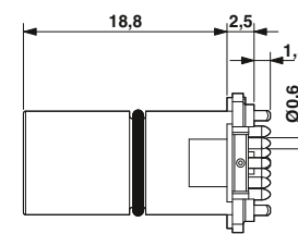
M12 plug contact carrier, straight, 12, 17-pos.
