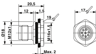
M12 pin, M16 fastening thread, solder cups
