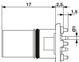
M12 socket contact carrier, straight, 4, 5-pos.
