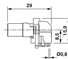
M12 socket contact carrier, angled, 17-pos.
