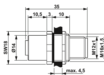
Control cabinet feed-through, socket to pin on both sides
