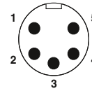
Plug, 5-pos.
