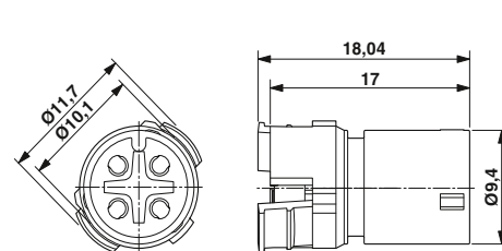
M12 contact carrier
