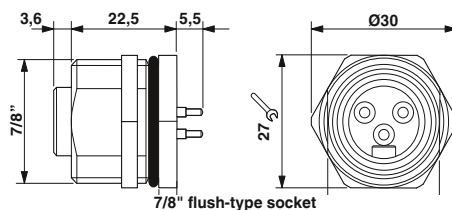
7/8" flush-type socket
