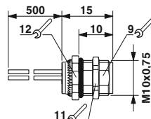
M8 flush-type socket, M10 fastening thread
