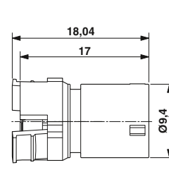
M12 contact carrier
