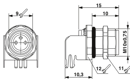
M8 flush-type socket, angled
