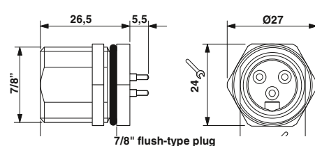
7/8" flush-type plug
