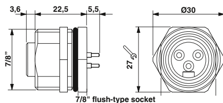
7/8" flush-type socket
