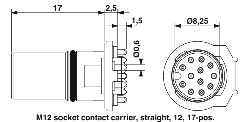
M12 socket contact carrier, straight, 12, 17-pos.
