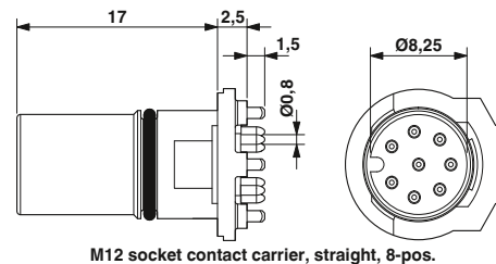
M12 socket contact carrier, straight, 8-pos.
