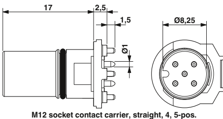
M12 socket contact carrier, straight, 4, 5-pos.
