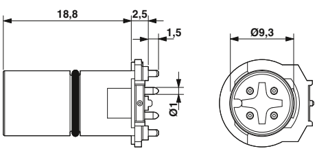
M12 plug contact carrier, straight, 4, 5-pos.
