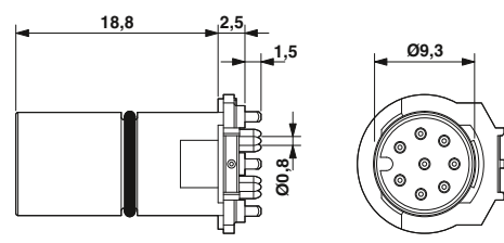
M12 plug contact carrier, straight, 8-pos.
