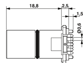
M12 plug contact carrier, straight, 12, 17-pos.
