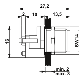
M12 flush-type plug, straight,
