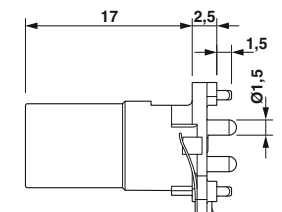
M12 flush-type socket
