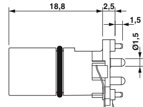
M12 flush-type plug
