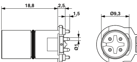
M12 plug contact carrier, straight, 4, 5-pos.
