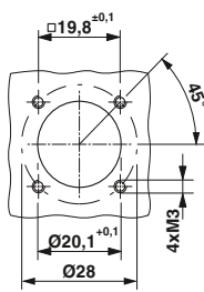
Installation dimensions
