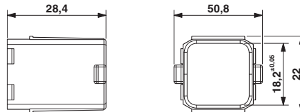
Dimensional drawing
