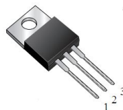
TO-220AB PS10U45CT
