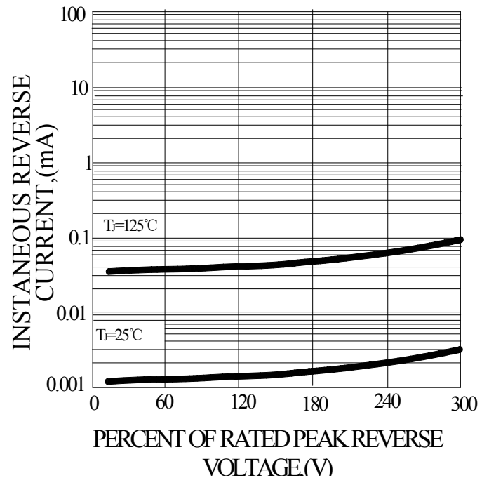
FIG.4-TYPICAL REVERSE CHARACTERISTICS
