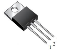
TO-220AB PSM20U60CT
