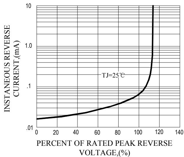
FIG.4-TYPICAL REVERSE CHARACTERISTICS
