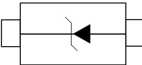
Circuit and Pin schematic
