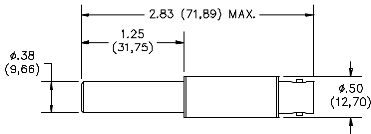
STANDARD WECO/BNC ADAPTER (4X MODEL 5008)
