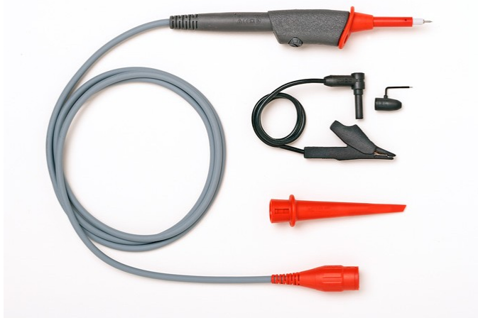
72940-2, X10 Insulated, 500 MHz, Red (additional photos on page 2)
