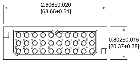
PLC 30
