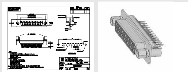
2-D Drawing
