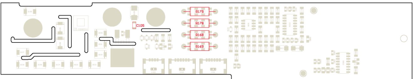
Fig. 2: Assembly drawing of 1SP0340D2S0 with highlighted gate resistors and gate capacitor
