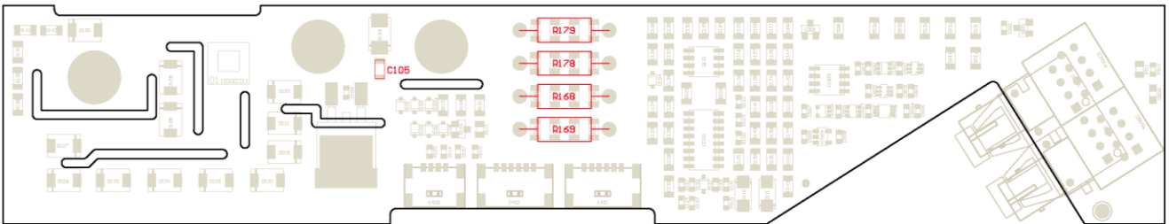
Fig. 1: Assembly drawing of 1SP0340V2M0 with highlighted gate resistors and gate capacitor
